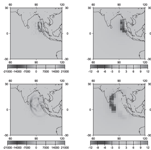
Fig. 7: Ocean bottom pressure and induced vertical displacements computed from predicted sea surface heights. Upper diagrams: 30 minutes after the earthquake, lower diagrams: 2 hours after the earthquake. Left: ocean bottom pressure in Pa; right: vertical displacement of the solid Earth's surface in mm.
