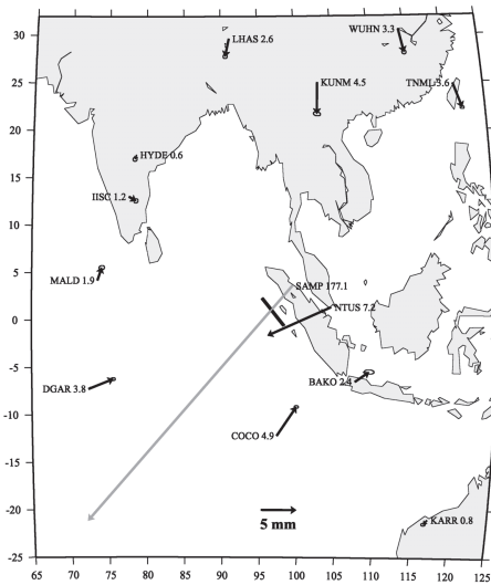
Fig. 6: Co-seismic displacements for Event B. The grey arrow for SAMP is scaled down by a factor of four. The offsets for SAMP and NTUS are determined with the inclusion of the post-seismic deformation term.
