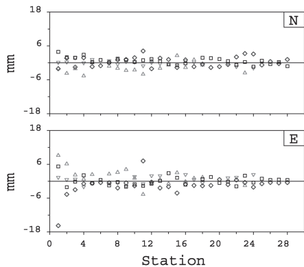
Fig. 3: Comparison of the computed offsets. For each station, the deviation from the mean of all estimates are shown for the east (lower) and north offsets. Triangles: Banerjee et al. (2005), inverted triangles: Vigny et al. (2005), squares: Kreemer et al. (2005), diamonds: this study.
