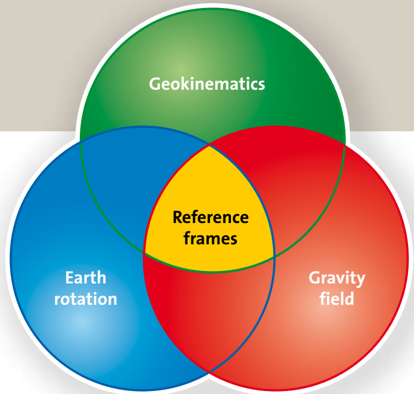
▲ Fig. 1: The observations in the so-called “three pillars” of geodesy, Earth's geometry, gravity field and rotation, are intrinsically interlinked and affected by the same unique Earth system processes. Together, these observations provide the basis to maintain the geodetic reference frames with high accuracy, spatial resolution and temporal stability.
