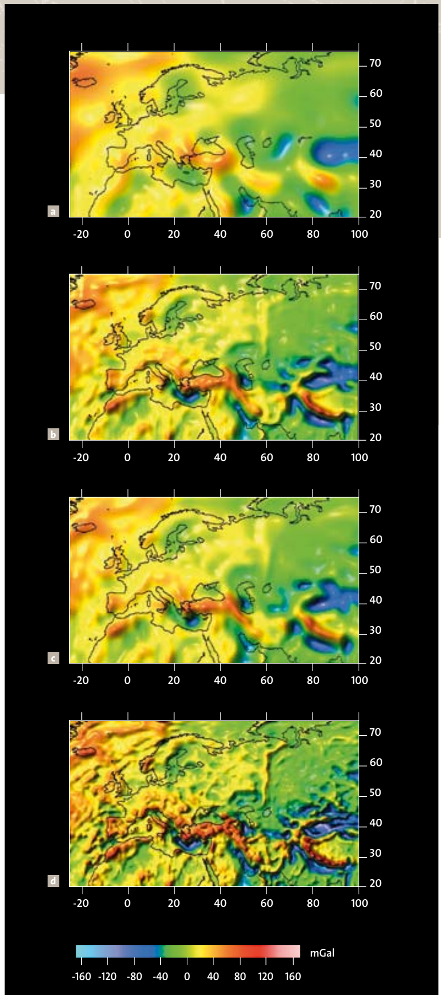
Fig. 3: Improvement of the Earth's gravity field models. These are (from top to bottom): a) GRIM-5S1 (best gravity field model before CHAMP and GRACE, computed from SLR data only); b) EIGEN-CHAMPo3S (gravity field from CHAMP); c) EIGEN-GRACEo3S (gravity field from GRACE); d) EIGEN-CGo3C (gravity field from GRACE combined with terrestrial data).
