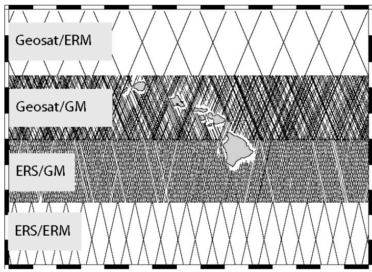
Figure 3. Ground tracks for two radar altimeters that have provided adequate coverage of the ocean surface. This is a 1500-km by 1000-km area around Hawaii. Geosat/ERM (US Navy) is the exact repeat orbit phase of the Geosat altimeter mission (US Navy, 1985-89). These ground tracks repeat every 17 days to monitor small changes in ocean surface height caused by time-varying oceanographic effects. Geosat/GM ground tracks were acquired during a 1.5-year period when the orbit was allowed to drift.
