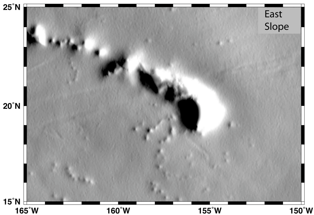
Figure 5. East component of sea surface slope \eta(x) derived from Geosat and ERS altimeter profiles. Note this component is rather noisy because the altimeter tracks (Figure 3) run mainly in a N-S direction.
