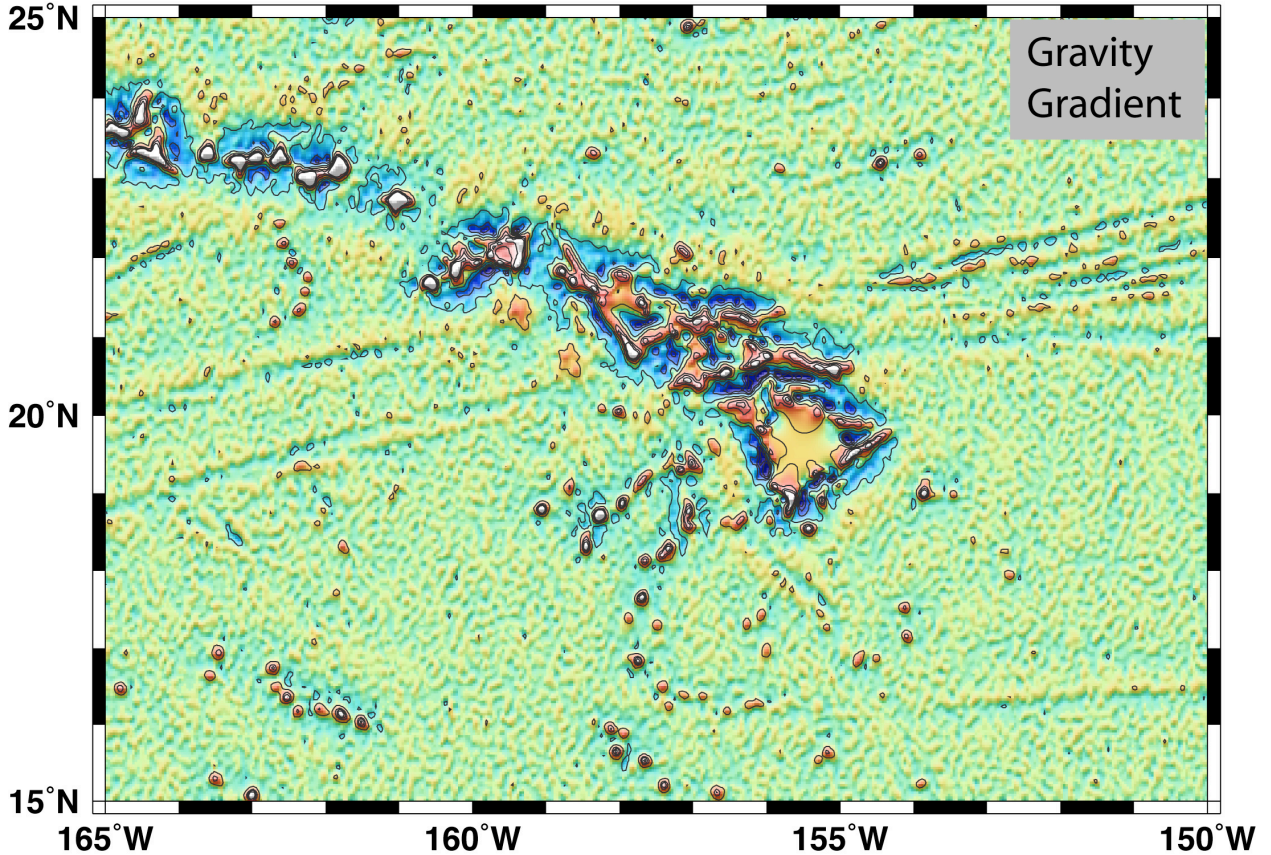
Figure 8. Vertical gravity gradient dg(\mathbf{x})/\delta z derived from east and north components of sea surface slope using equation (15). Note this second derivative of the geoid amplifies the shortest wavelengths; compare with the original geoid (Figure 3). Noise in the altimeter measurements has been amplified resulting in an artificial texture. (100 Eotvos contour interval)
