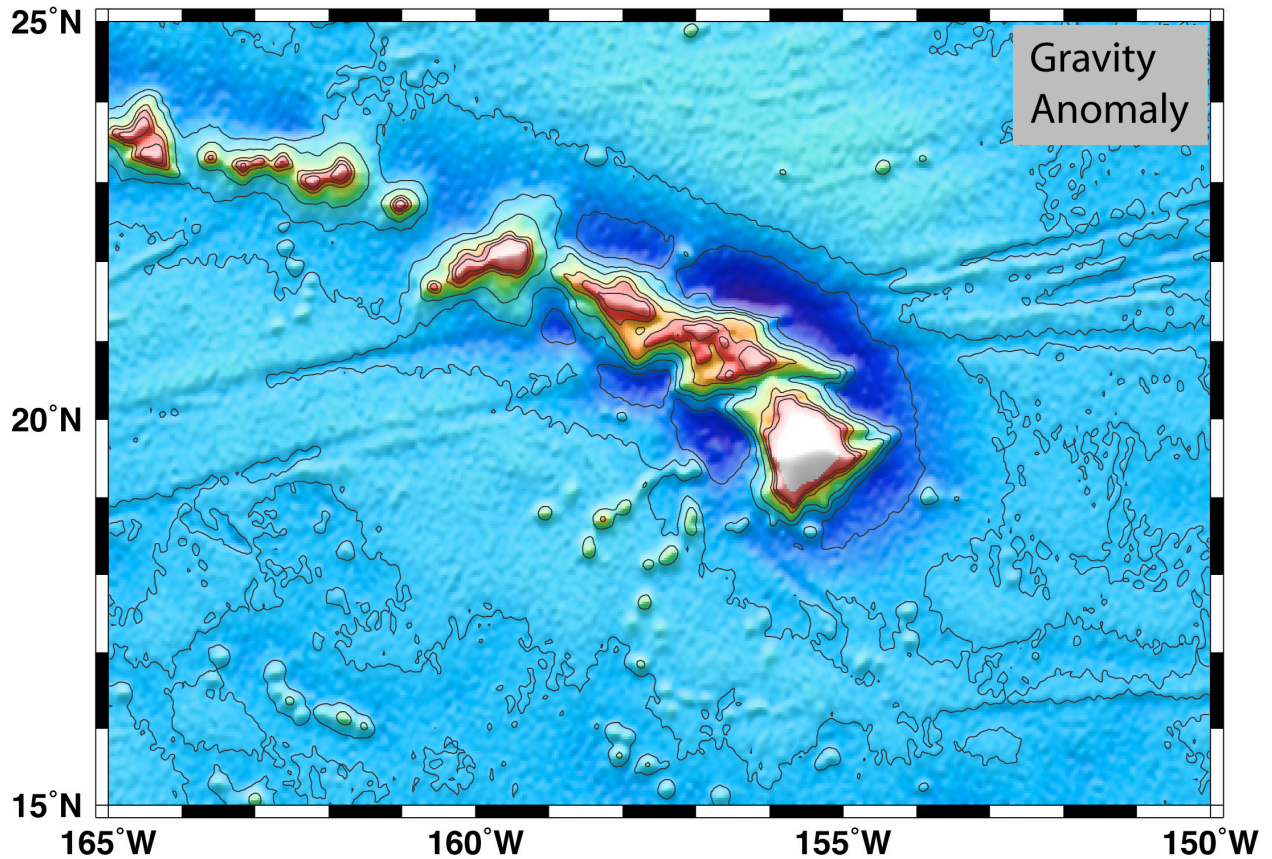
Figure 7. Gravity anomaly \Delta g(\mathbf{x}) derived from east and north components of sea surface slope using equation (14). (50 mGal contour interval)
