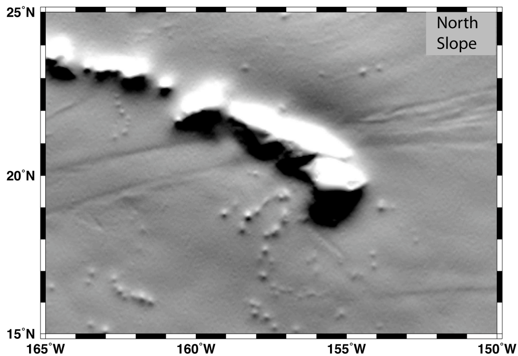
Figure 6. North component of sea surface slope \xi(x) derived from Geosat and ERS altimeter profiles. Note this component has lower noise because the altimeter tracks (Figure 3) run mainly in a N-S direction.
