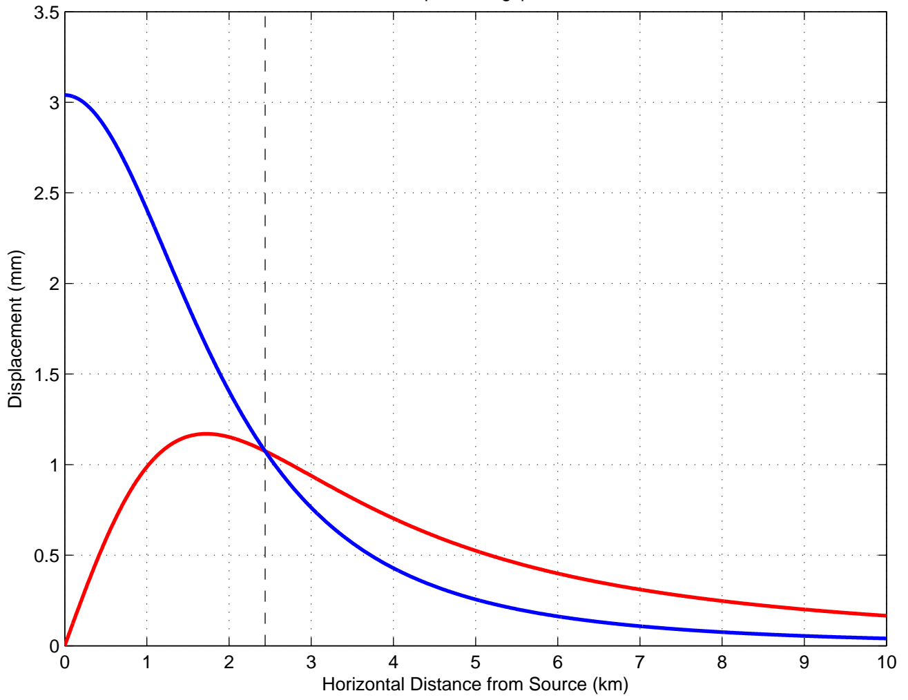
Expected Surface Displacement Red=Horizontal, Blue=Vertical Dashed=depth of Mogi point source
